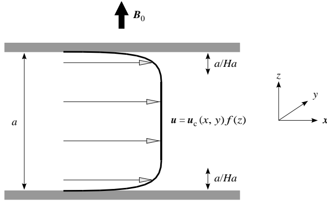
FIGURE 1. Hartmann layers form on walls perpendicular to the imposed magnetic field B_0 . The core velocity u_c decays to zero over a distance a/Ha = \sqrt{\rho\eta_*\nu}/B_0 to satisfy the no-slip boundary condition on the walls.
