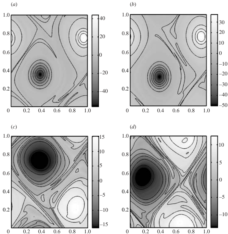
FIGURE 7. The vorticity at the later time t = 5.0 for the same four equations and parameter values as figure 6.
